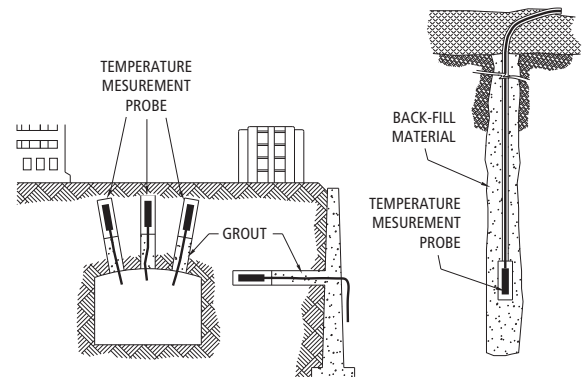
TH Probe Typical Installations
